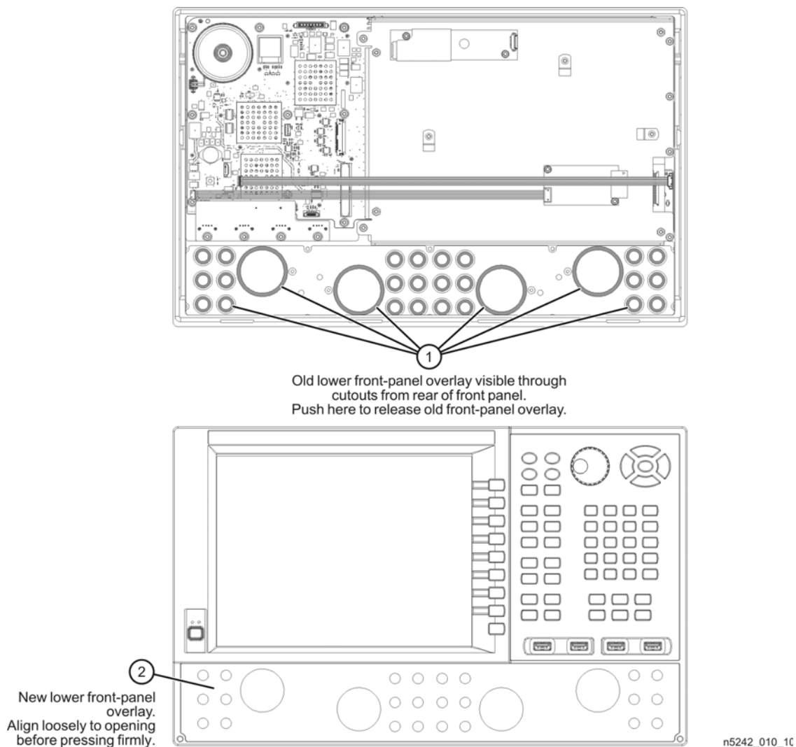
Figure 16 Lower Front Panel Overlay Replacement
