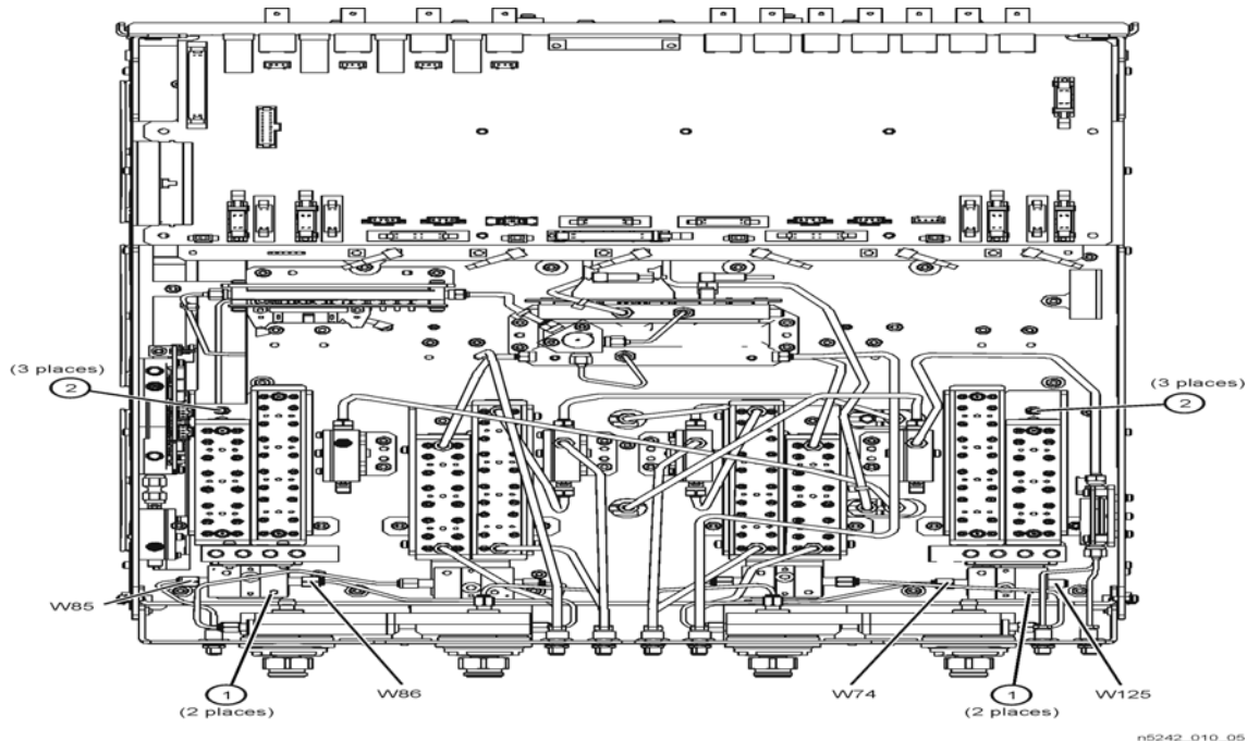
Figure 7 New Brackets Installation into the Analyzer
