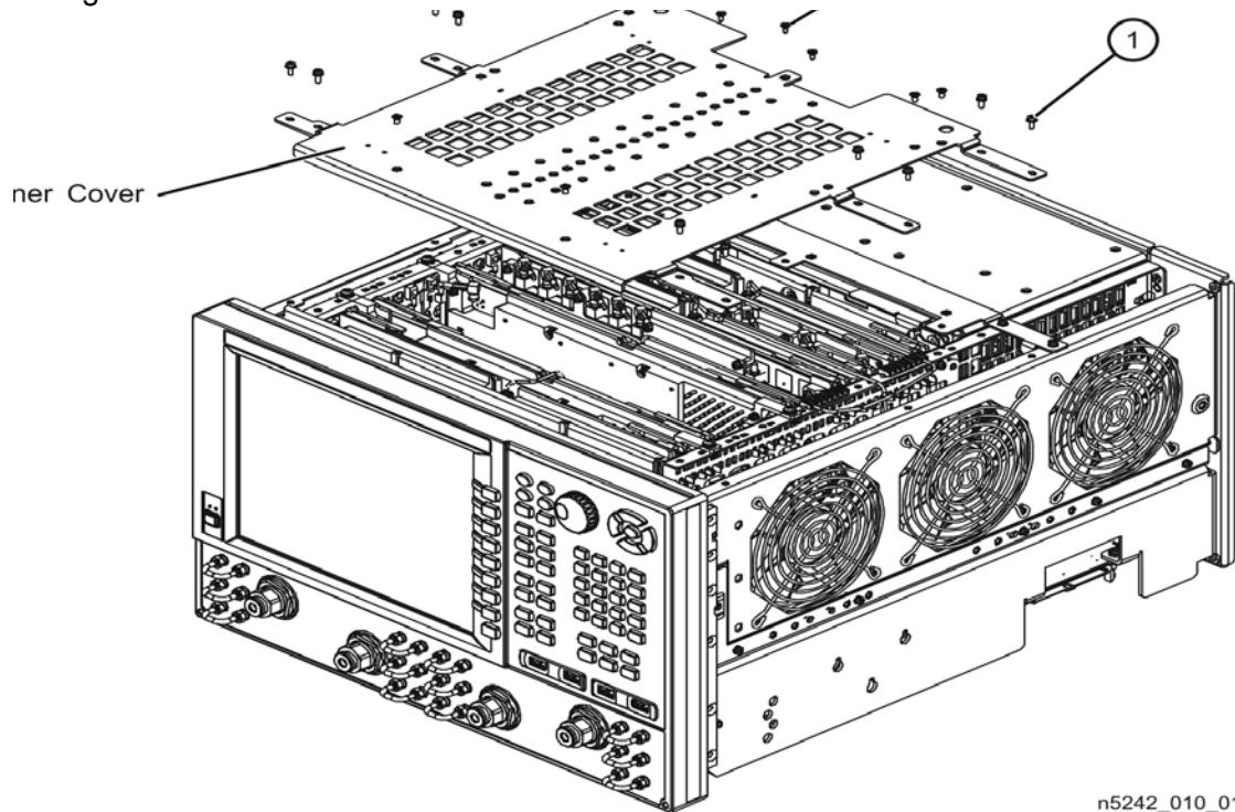
Figure 18 Inner Cover Reinstallation
